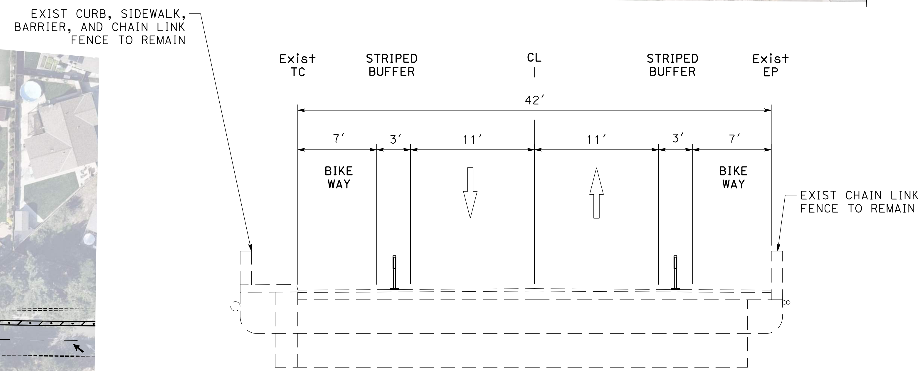
SECTION B-B SEGMENT 2 MUIRWOOD DR TO PAYNE RD SCALE: 1" = 5'
