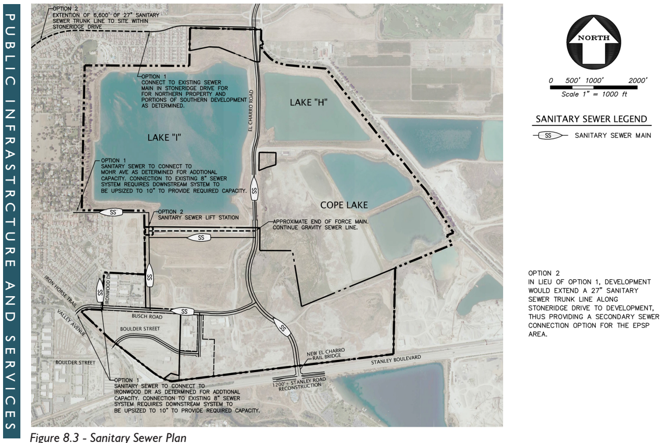
Figure 8.3 - Sanitary Sewer Plan
