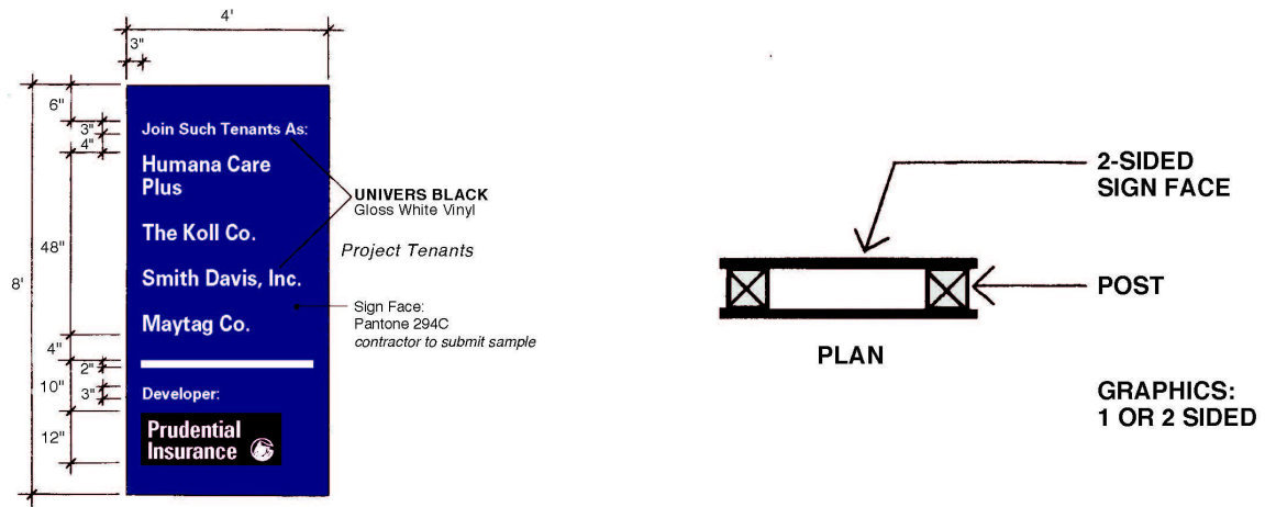
Figure 4-5: Temporary Multi-Tenant Building Signs
