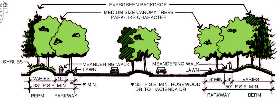
TYPICAL SECTION
